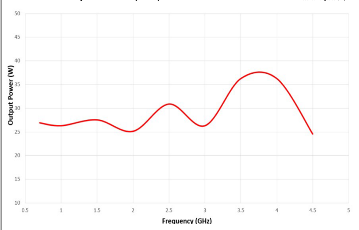
8000-071 Output Power (1dB)
